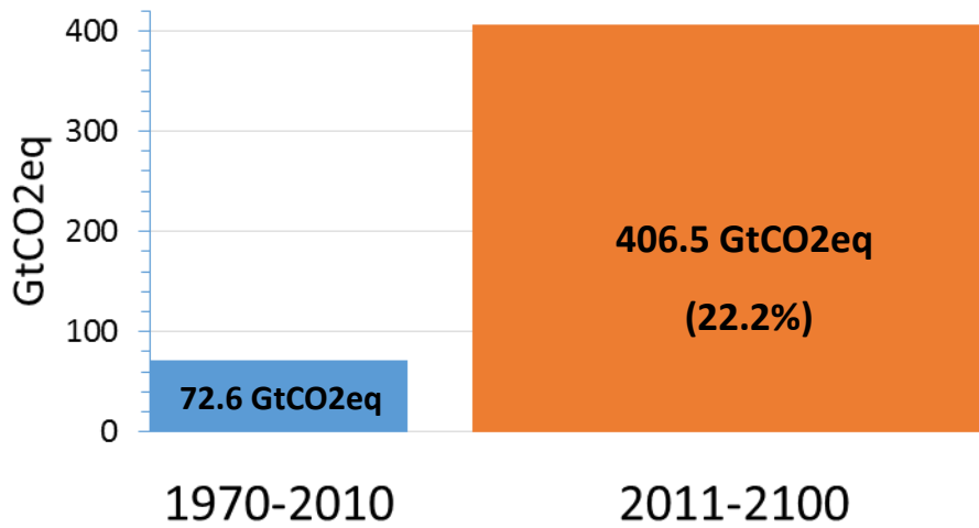
Future (2011-2100) Carbon Budget allocated by MCJ-RCP2.6
